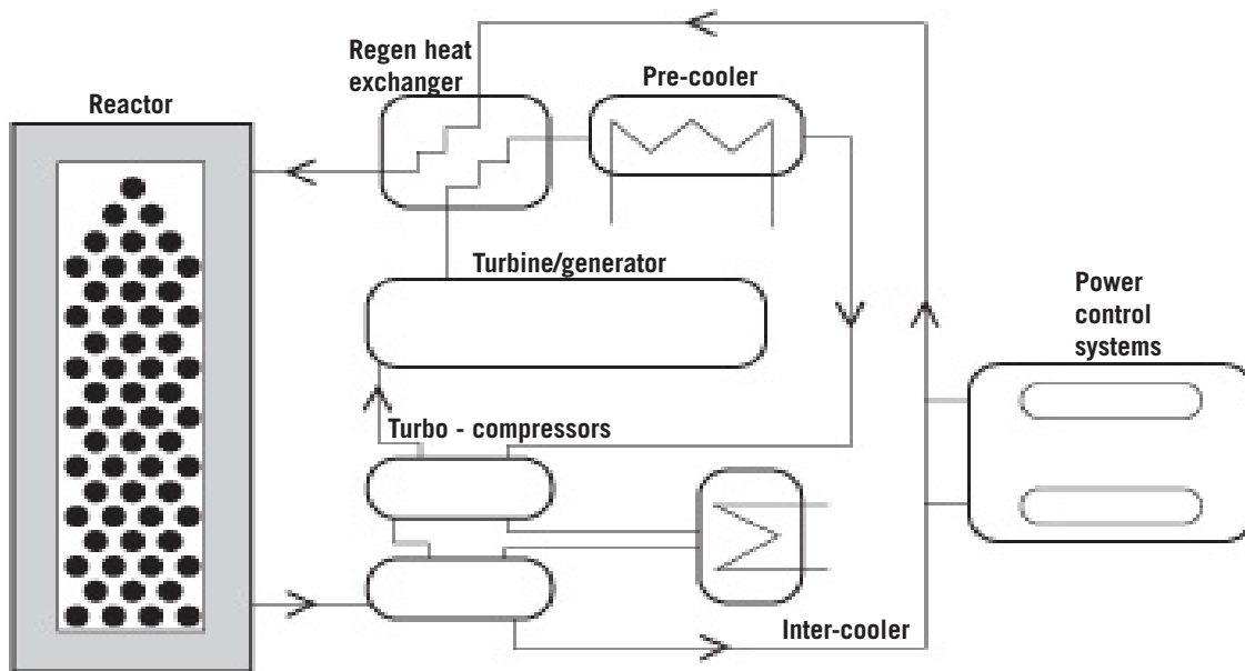
Figure 8: Circuit of Pebble Bed Modular Reactor
